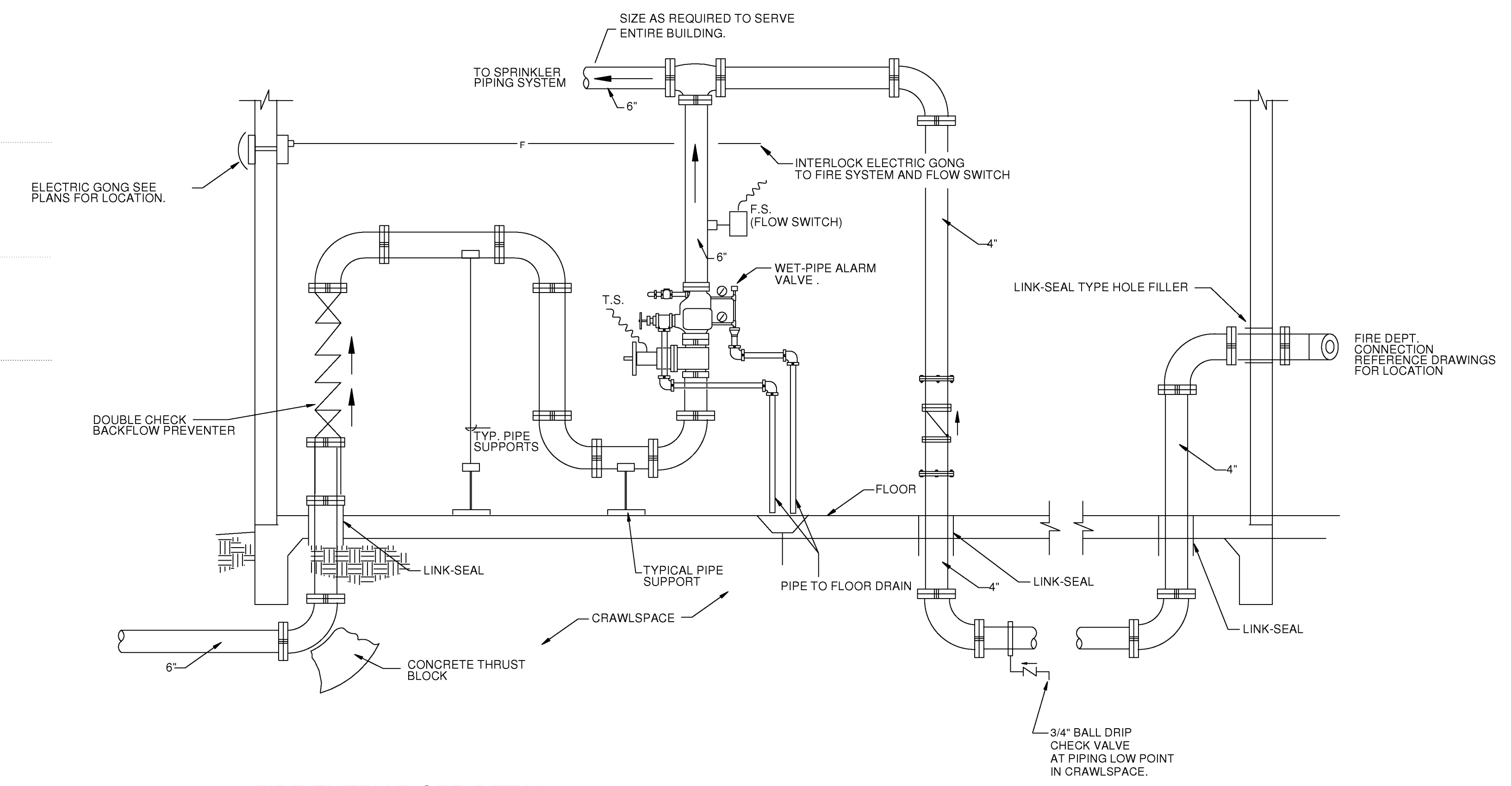
2 FIRE ENTRY/RISER DETAIL NOT TO SCALE
